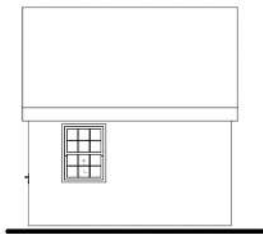
NORTH ELEVATION 1:100
